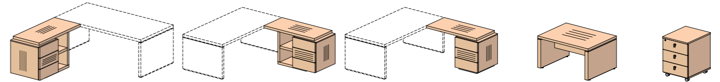
46T800 1280x668x748 46T810 1280x668x748 46T801 1280x668x748 46S850 800x600x450 46T820 408x500x557
