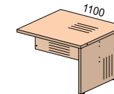
64B002 1155x1000x745
