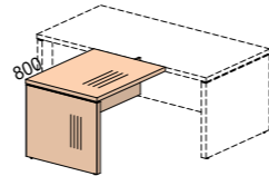
64B004 949x800x745
